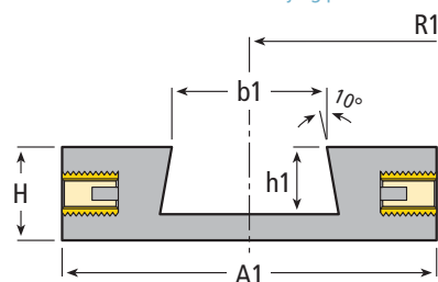
Obere Platte | Carrying plate
